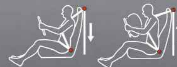
Pretensioner with Load Limiter Seat Belt
